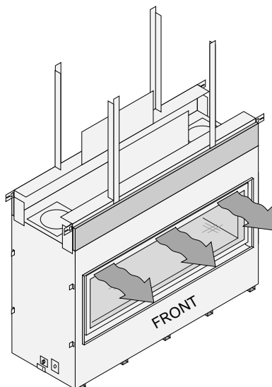
Air Flow to Front
