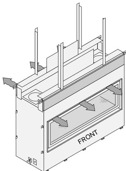
Divided Air Flow (stock)
